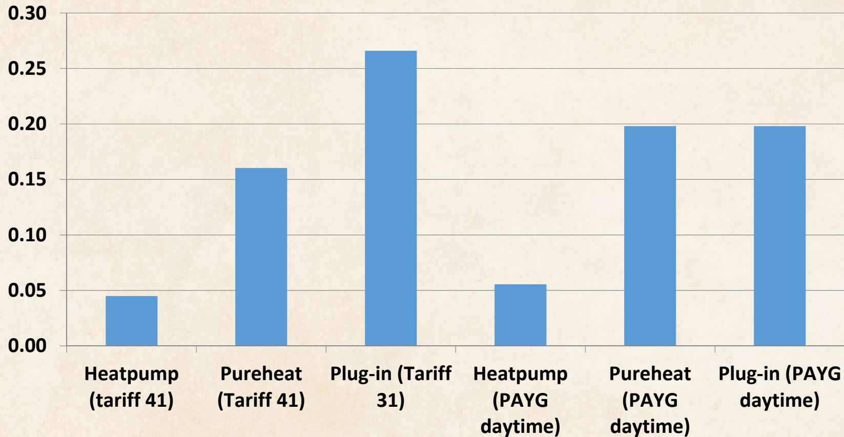
Cost per kWh of delivered heat
