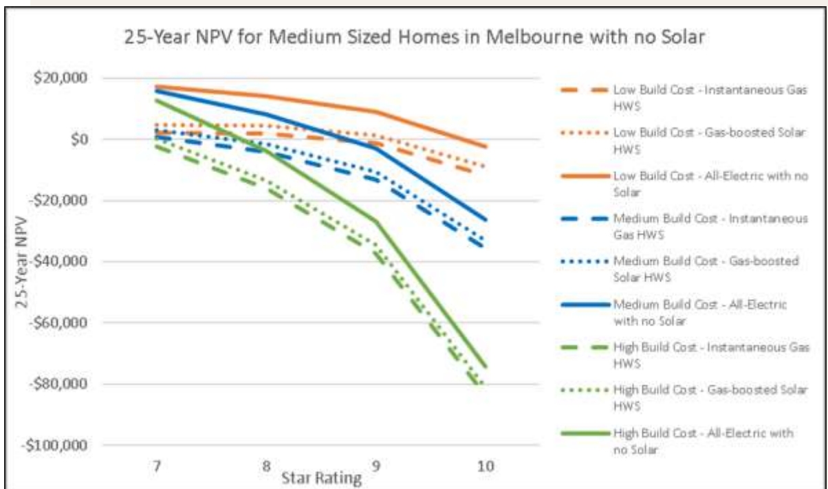
Figure 38: 25-Year NPV of All-Electric versus Dual Fuel Home, Melbourne, no Solar PV (7% Discount, Medium Build Cost Premium) 71
